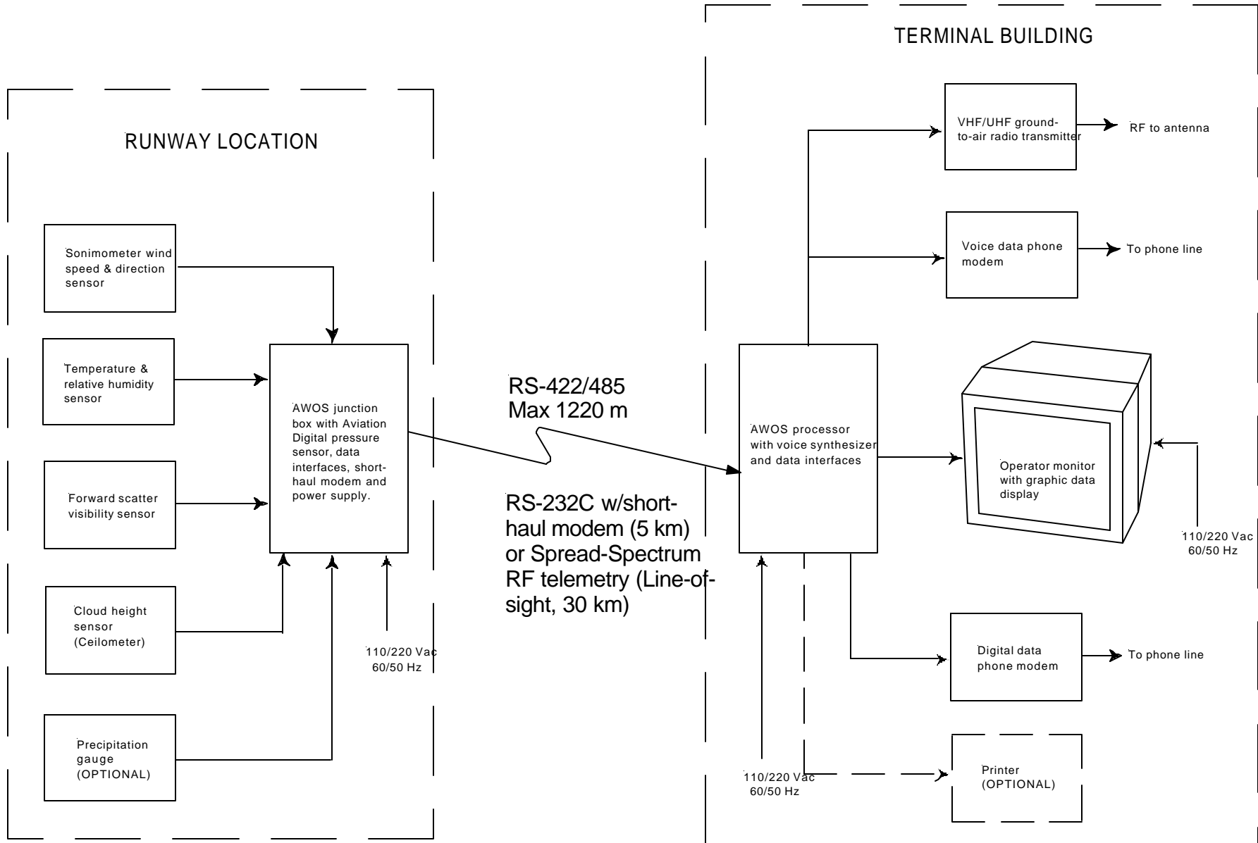
AWOS III FUNCTIONAL BLOCK DIAGRAM
